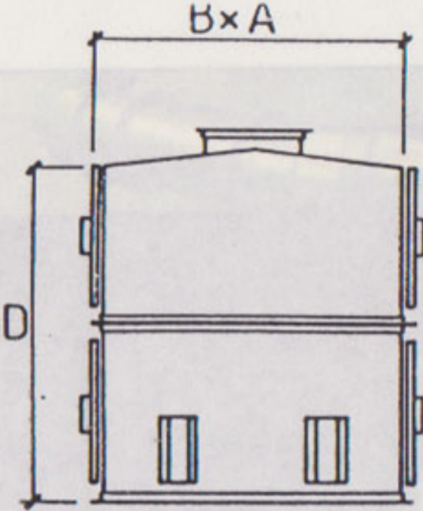
FLANGE MOUNTING With FAN FX 1000 to FX 1650
