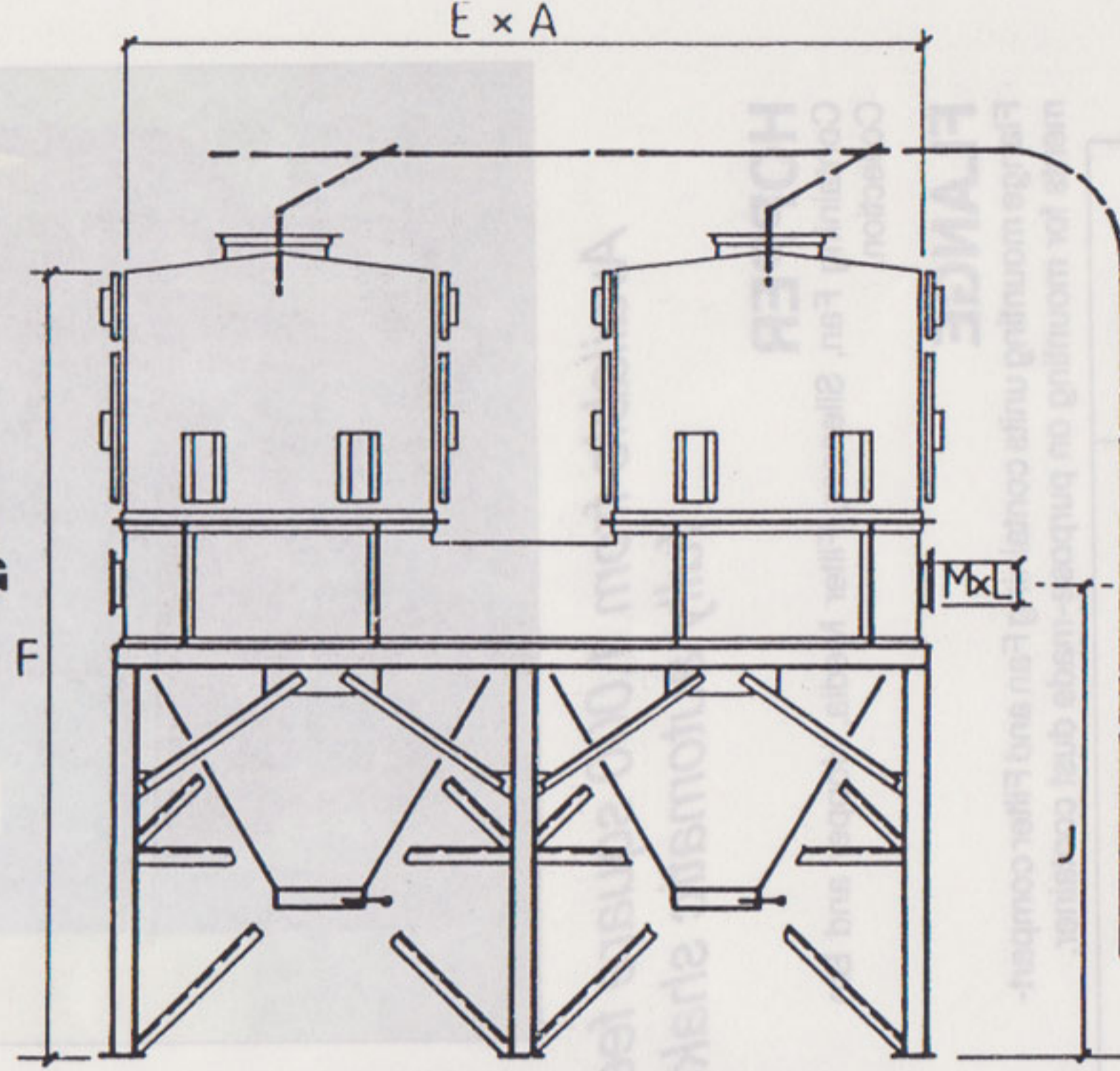
VALLEY HOPPER VALLEY HOPPER with FLOOR MOUNTING FAN FX 1000 to FX 3300
